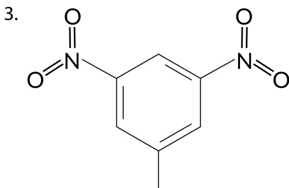
1-methyl-3,5-dinitrobenzene
