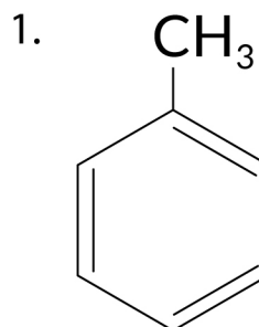
Toluene
