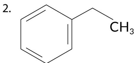
Ethyl Benzene
