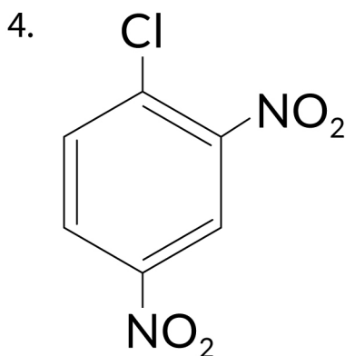
2,4-Dinitrochlorobenzene
